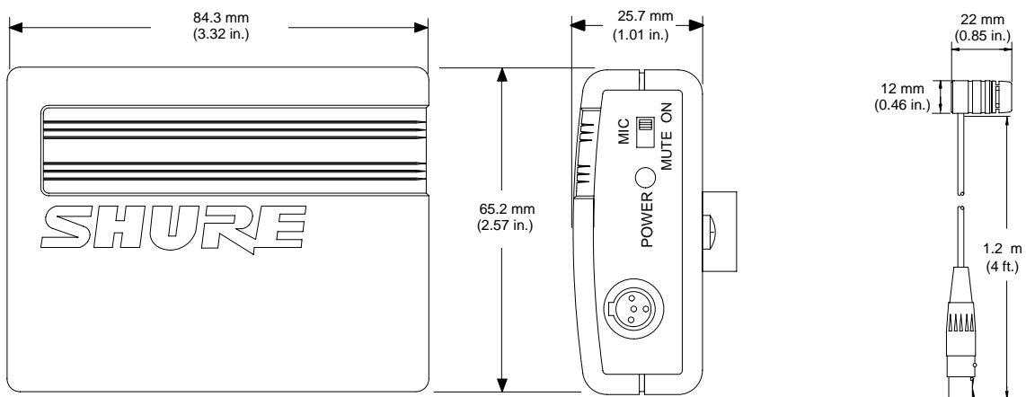
DIMENSIONS Figure 3
