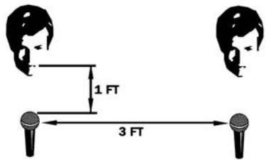
3-to-1 Rule
