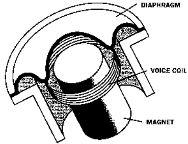
Dynamic Microphone
