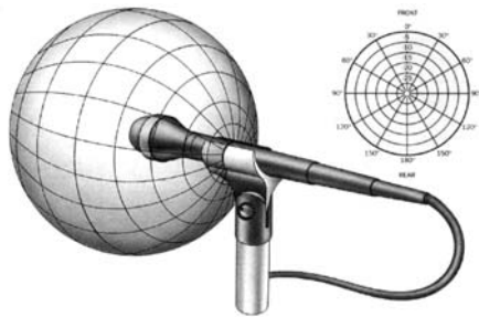
Omnidirectional Microphone
